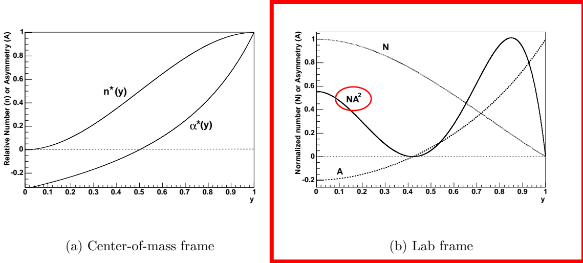
FIG. 1: Relative number and asymmetry distributions versus electron fractional energy y in the muon rest frame (left panel) and in the laboratory frame (right panel). The differential figure-of-merit product NA^2 in the laboratory frame illustrates the importance of the higher-energy electrons in reducing the measurement statistical uncertainty.
