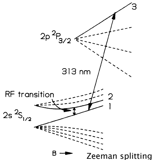
FIG. 2. Diagram of the energy levels of {}^9\text{Be}^+ in a magnetic field B . The states labeled 1, 2, and 3 correspond to those in Fig. 1.
