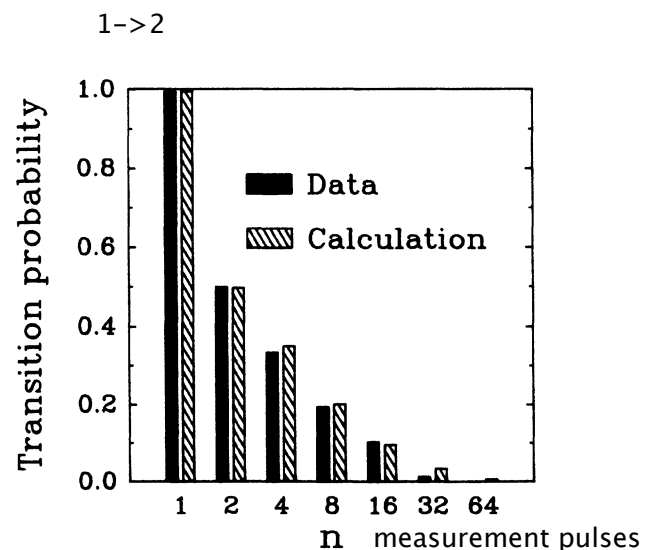
FIG. 3. Graph of the experimental and calculated 1 \rightarrow 2 transition probabilities as a function of the number of measurement pulses n . The decrease of the transition probabilities with increasing n demonstrates the quantum Zeno effect.
