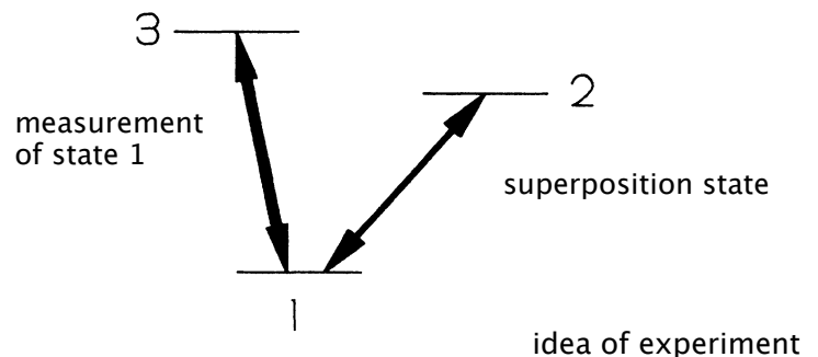
FIG. 1. Energy-level diagram for Cook's proposed demonstration of the quantum Zeno effect.
